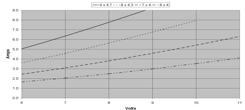
HC2212-1180 Current vs. Voltage with Propeller
